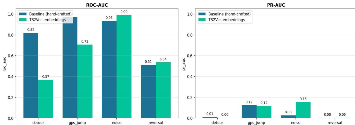
Baseline vs TS2Vec — anomaly detection performance
